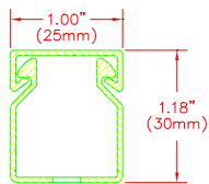
FRONT SECTION
